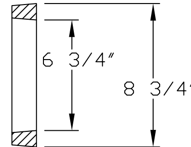
GRATE SECTION
