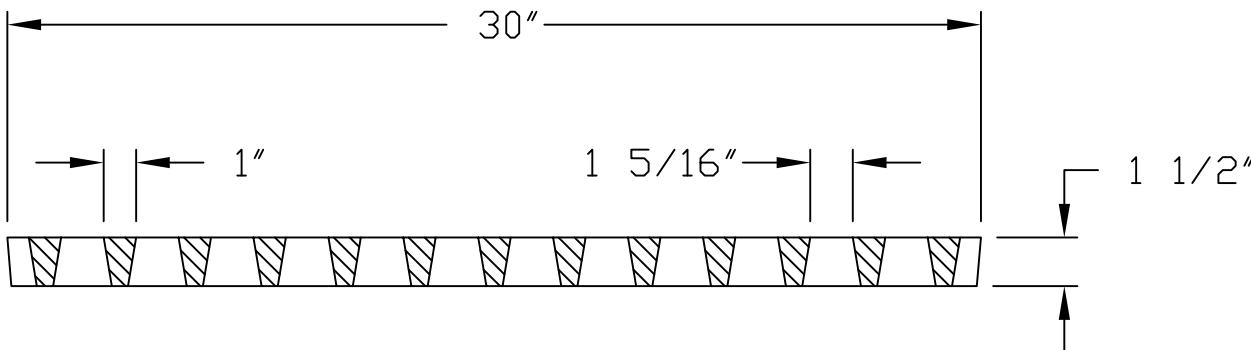
GRATE SECTION
